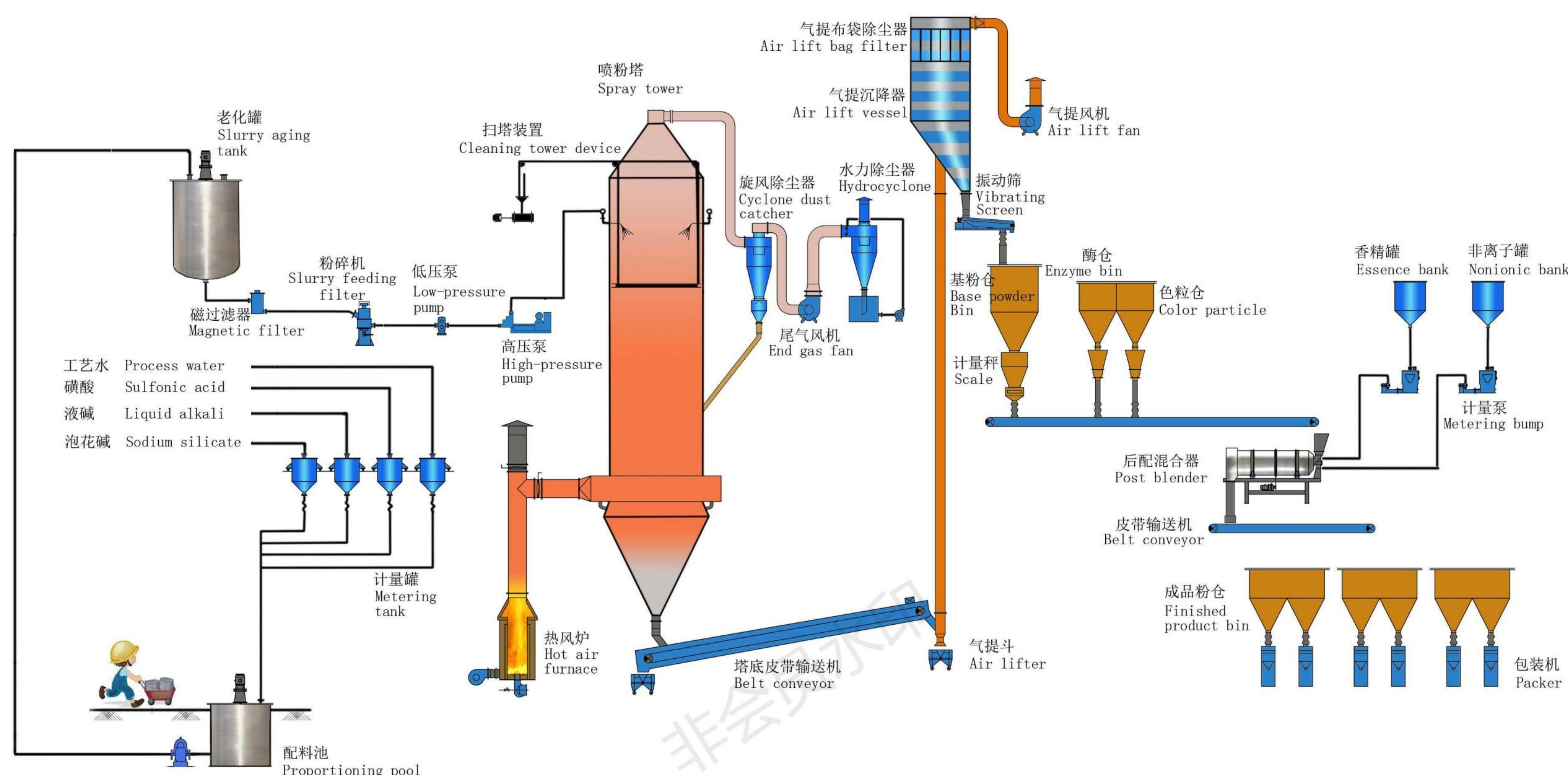
小产量洗衣粉生产线流程图 Flow diagram of washing powder production line with small output
