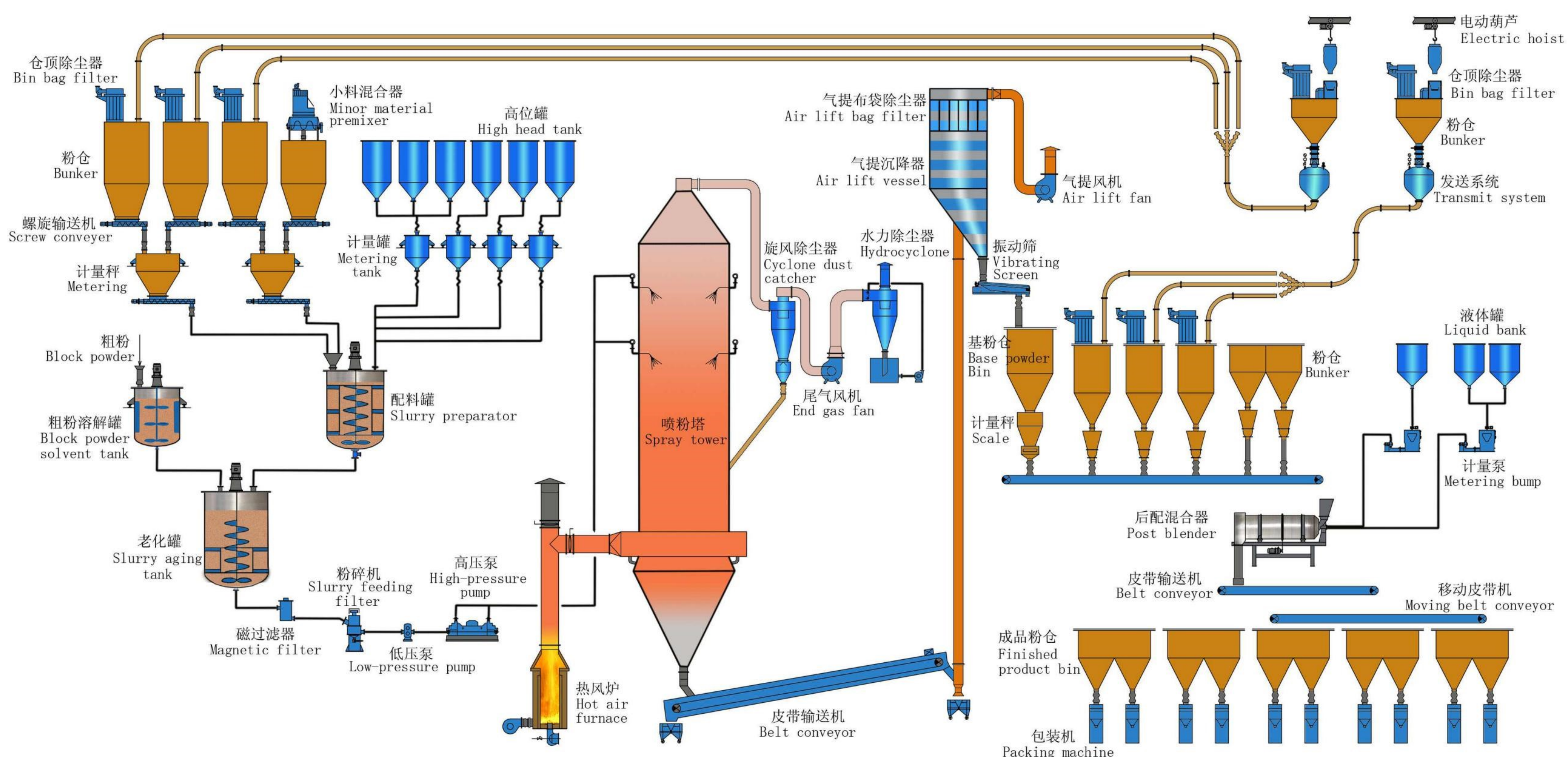
大产量洗衣粉生产线流程图 Flow diagram of washing powder production line with large output
